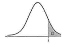
Right-tailed test
