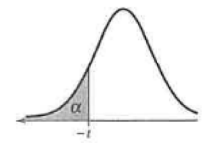
Left-tailed test
