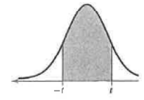
c-confidence interval
