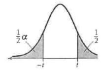
Two-tailed test
